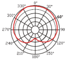
Figure 1: Polar pattern
